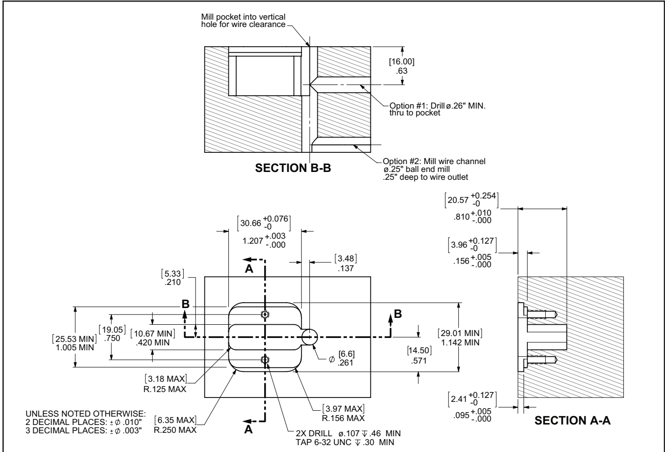
Switch Assembly Pocket Dimensions
